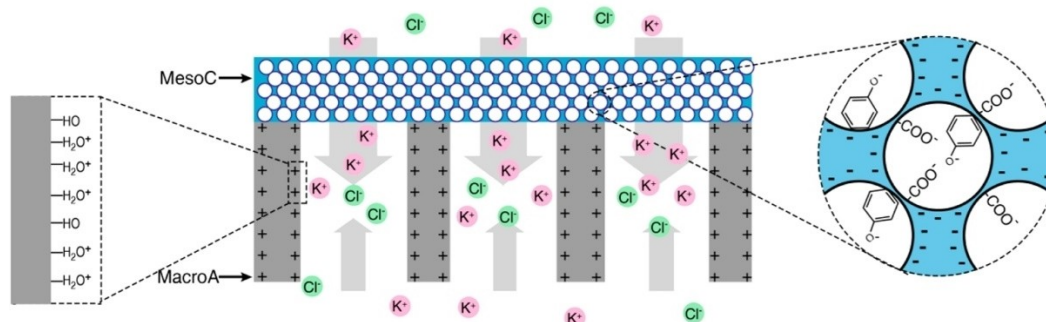
Fig. 23. Schematic representation of how the mesoporous carbon and macroporous alumina selectively allow ion transport to produce the diode effect. Reprinted with permission from [106]. Copyright (2012) American Chemical Society.
