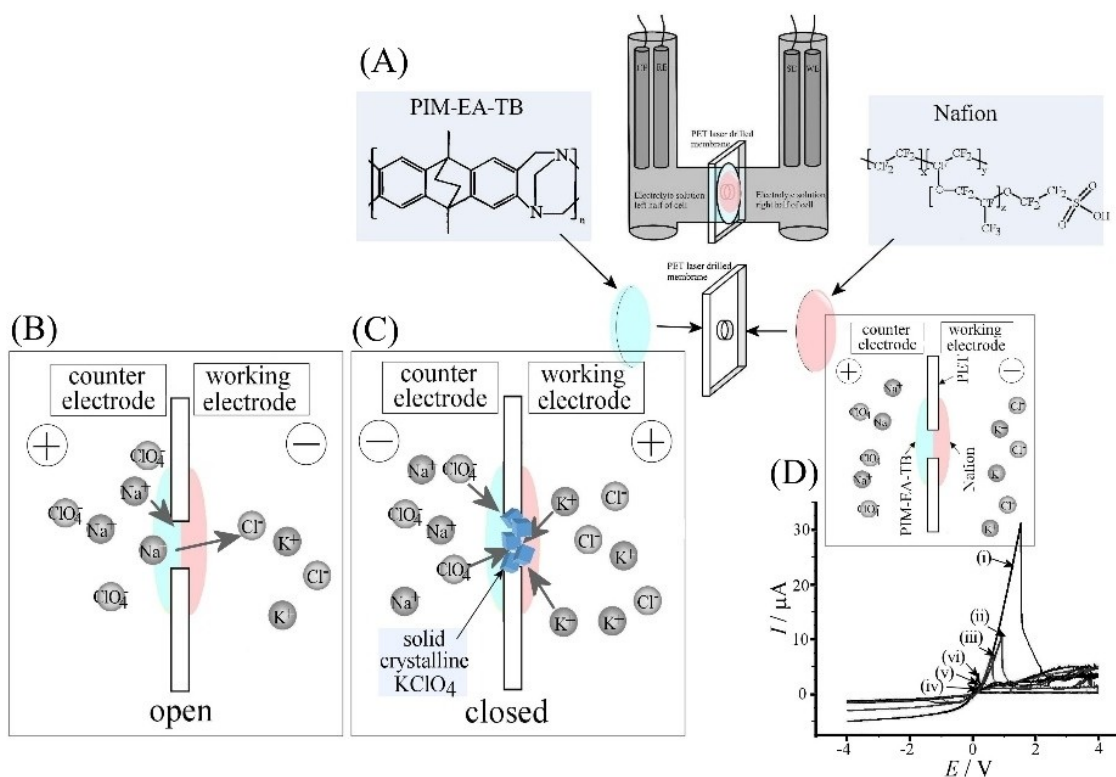
Fig. 21. (A) Schematic of the four-electrode measurement cell with PIM-EA-TB | Nafion heterojunction. (B, C) Schematic drawing of cation and anion transport leading to junction blocking when \text{KClO}_4 forms. (D) Cyclic voltammetry data (scan rate 25 \text{ mV s}^{-1} ) for the PIM-EA-TB | Nafion heterojunction on a 20 \mu\text{m} diameter microhole in PET immersed in aqueous KCl (with concentration (i) 0.1, (ii) 1.0, (iii) 10, (iv) 100, (v) 500, (vi) 1000 mM in the working electrode compartment) and aqueous \text{NaClO}_4 (with concentration 0.1 M in the counter electrode compartment). Reprinted with permission from [102]. Copyright (2017) Elsevier.
