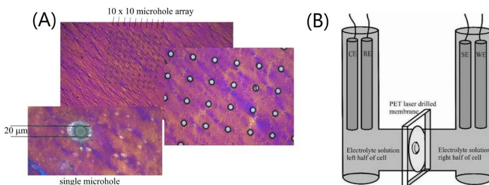
Fig. 12. (A) Optical micrograph showing a 20 \mu\text{m} thick PET substrate with a single microhole or a 10 \times 10 microhole array laser drilled with approx. 20 \mu\text{m} diameter. To produce ionic diode effects, one side of the PET film is coated with ionomer. (B) Experimental four-electrode electrochemical membrane cell. Reprinted with permission from [66]. Copyright (2020) Elsevier.
