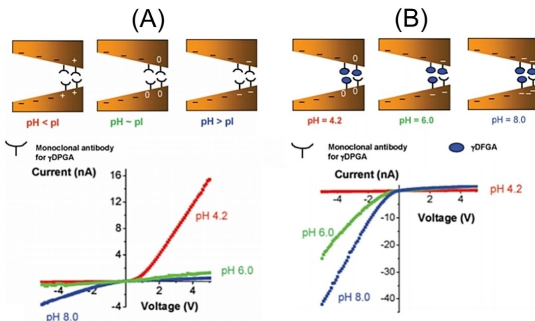
Fig. 20. (A) Effect of electrolyte pH on the monoclonal antibody for detection of the bacterial polyglutamic acid ( \gamma\text{DPGA} ). (B) Sensing \gamma\text{DPGA} with a nanopore that contained mAb F26G3 immobilised at the tip. At each pH value distinct ionic diode effects are generated. Reprinted with permission from [101]. Copyright (2009) American Chemical Society.
