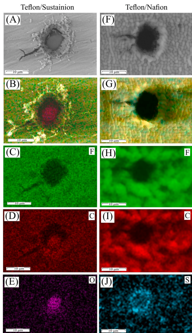
Fig. 4. (A) Scanning electron microscopy (SEM, backscatter) image of the backside of a Sustainion coated Tefflon film with 10 \mu\text{m} diameter microhole. (B–E) EDS mapping for F, C, O. (F) SEM image of the backside of a Nafion coated Tefflon film with microhole. (G–J) EDS mapping for F, C, S. Images (B) and (G) are layered X-ray images combining images C–D and H–J.
